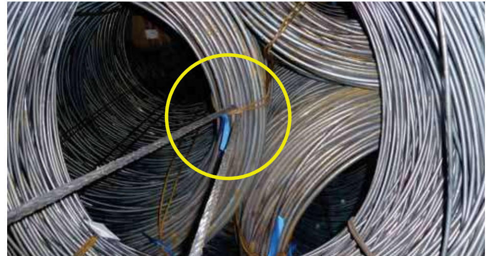
✗ The wires shall not be secured to the bundling wires of WRIC further back in the stow
